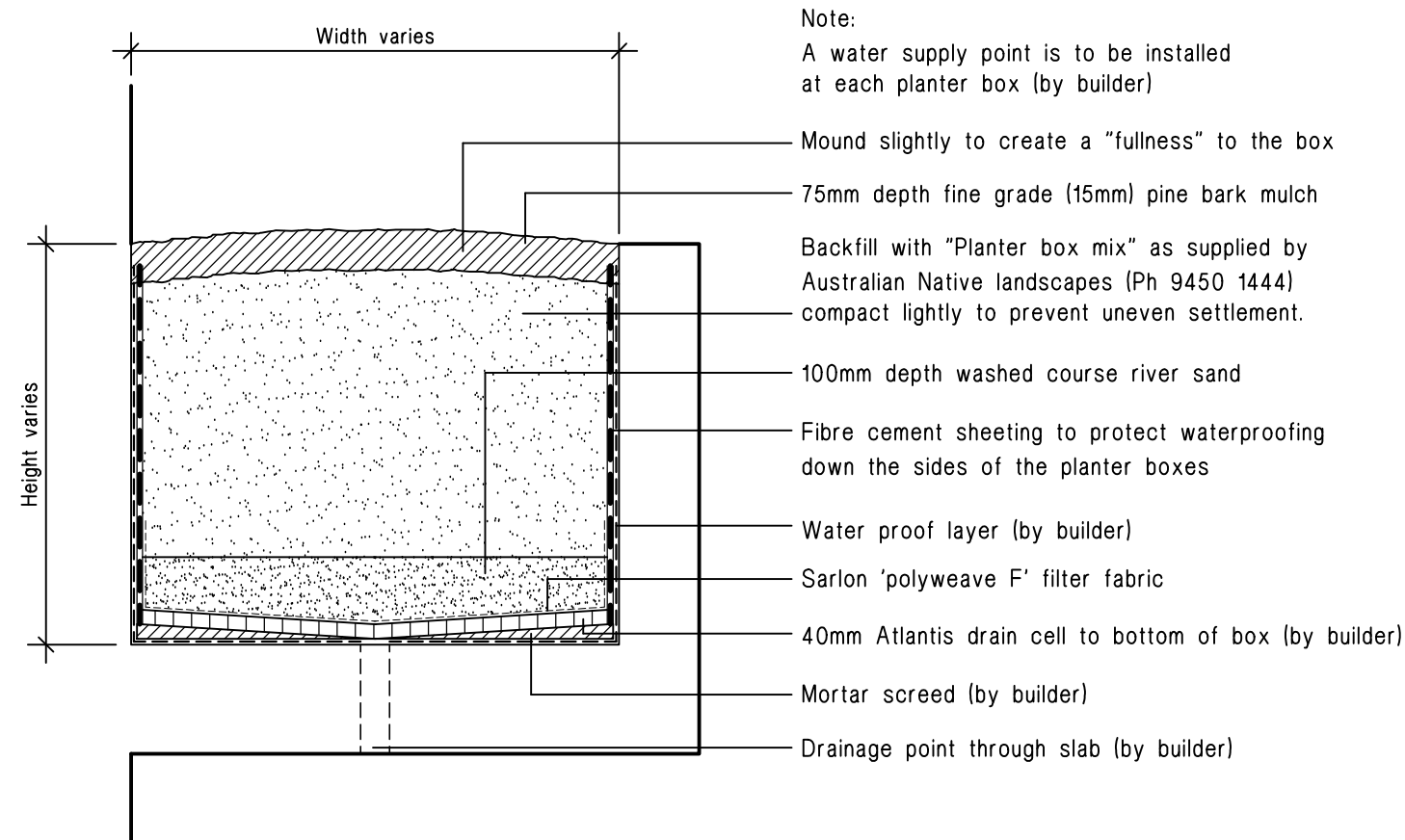
Typical planter box Detail.
